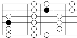
Dorian-2nd Position
