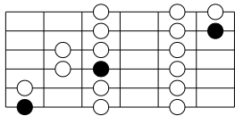
Ionian-1st Position
