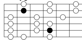
Phrygian-3rd Position
